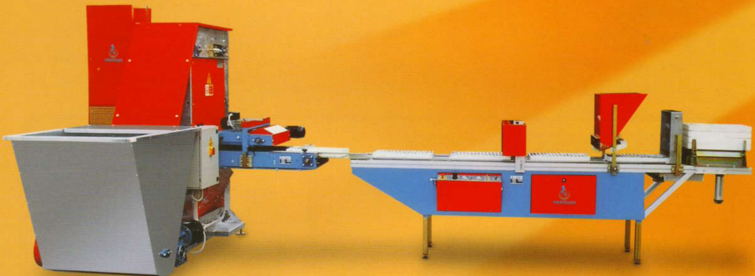
Linea di semina composta da riempitore Mod. RUS 65 e minilinea Mod. LSF Sowing line composed by trayfiller mod. RUS 65 and row seeding line mod. LSF.
